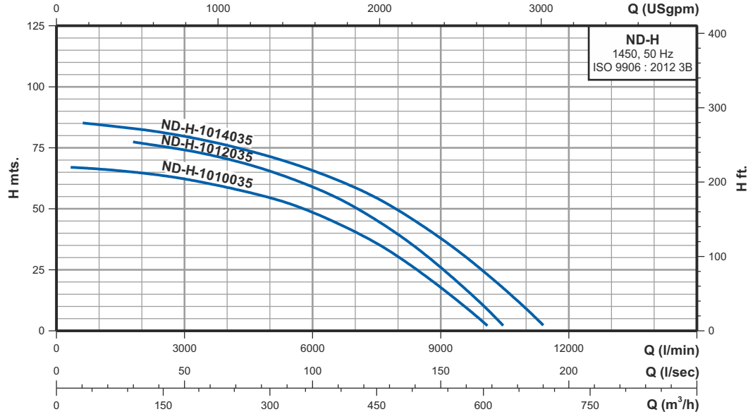
PERFORMANCE CHART AT n = 1450 RPM
