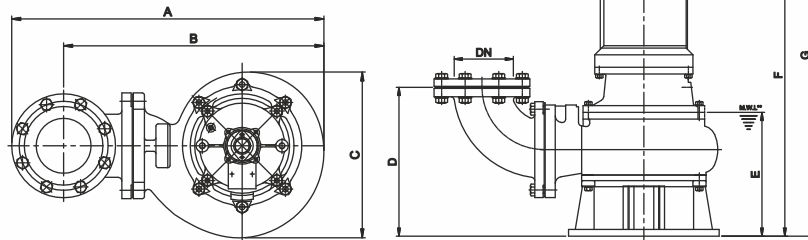
DIMENSIONS Figure 1
