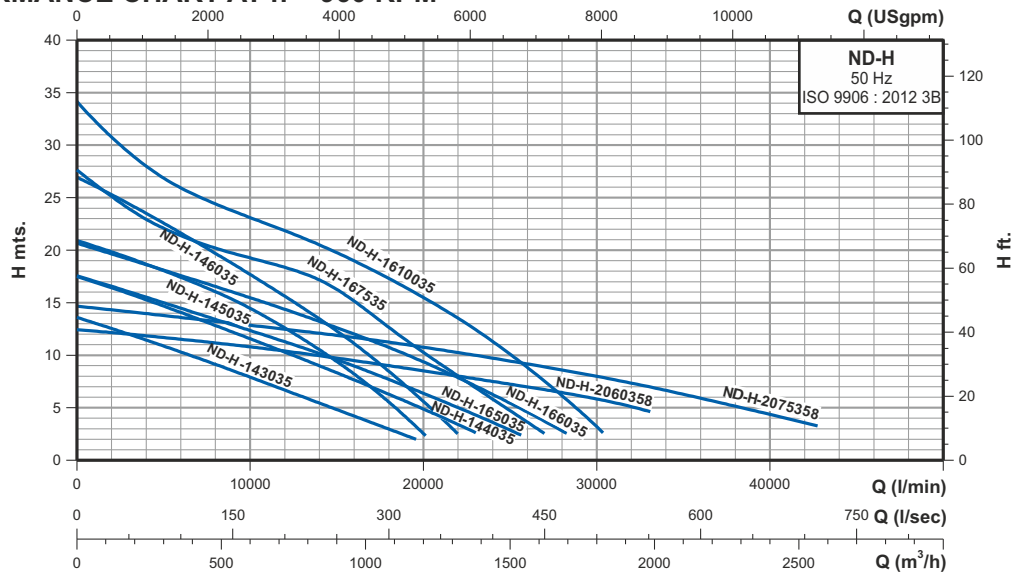
PERFORMANCE CHART AT n = 960 RPM
