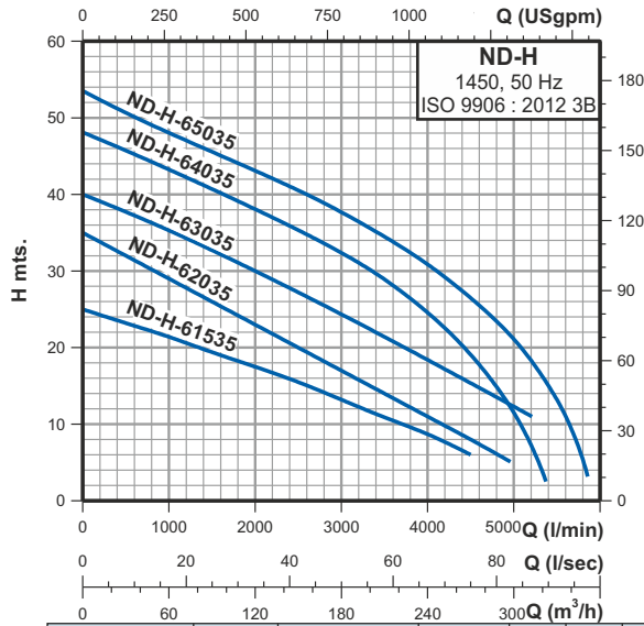
PERFORMANCE CHART AT n = 1450 RPM
