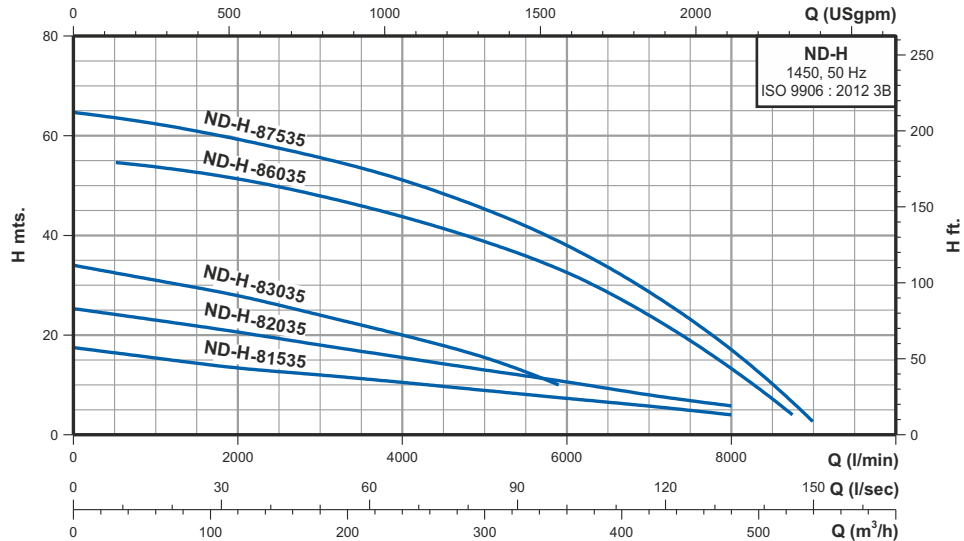
PERFORMANCE CHART AT n = 1450 RPM
