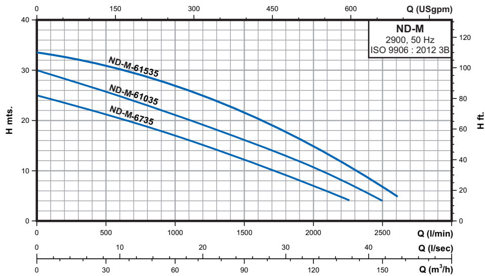
PERFORMANCE CHART AT n = 2900 RPM FOR CONSTRUCTION DRAINAGE PUMP
