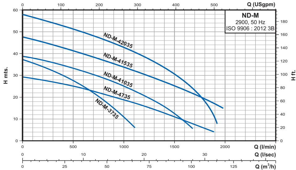
PERFORMANCE DATA AT n = 2900 RPM
