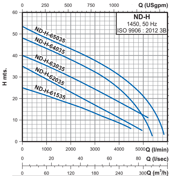
PERFORMANCE CHART AT n = 1450 RPM
